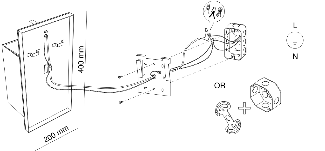
DIMENSIONI mm / DIMENSIONS mm
